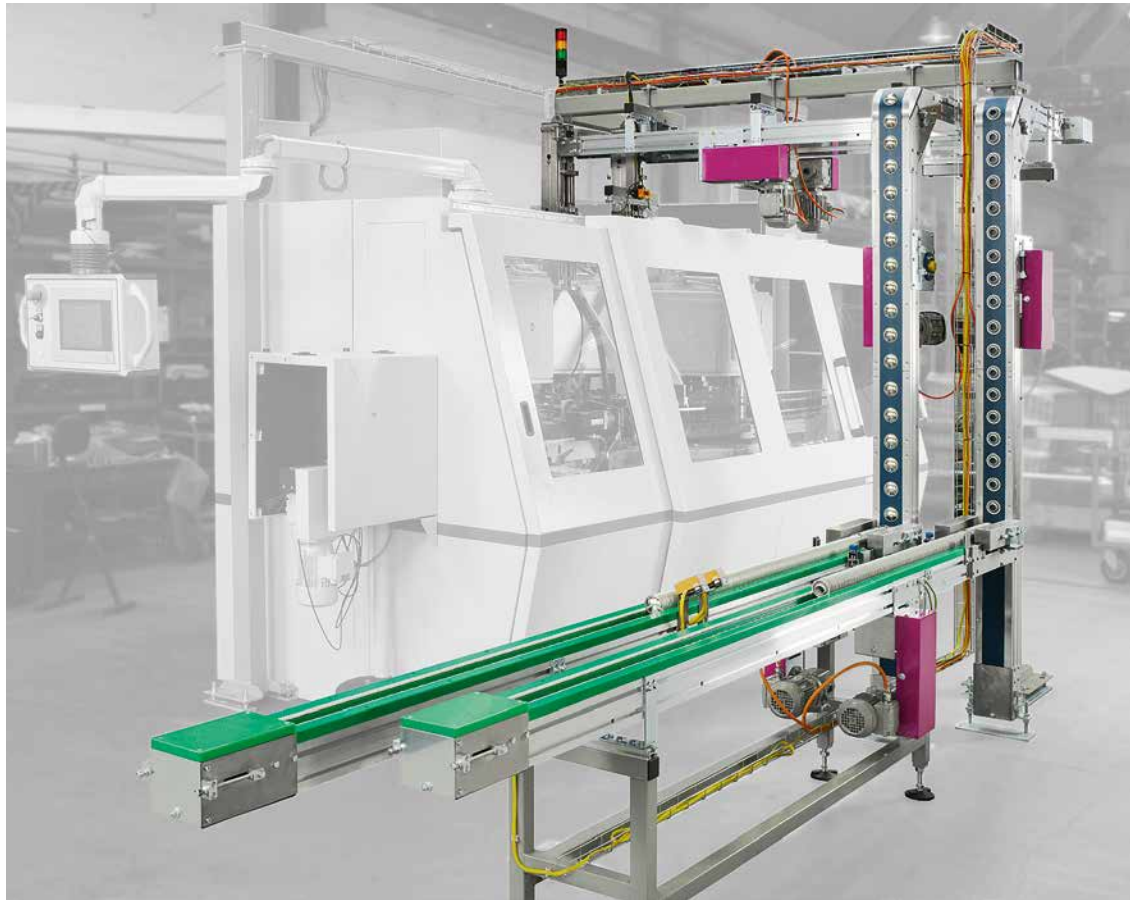
Feeding system for Aerosol Bottom and Domes
